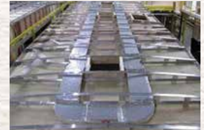
3" Aluminum floor studs, heat duct and 5/8" tongue and groove plywood floor.
